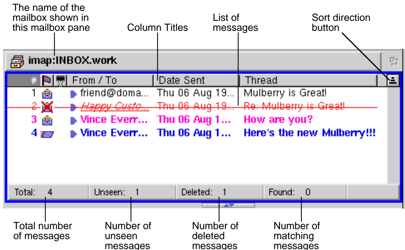
Figure 5 The Mailbox pane
