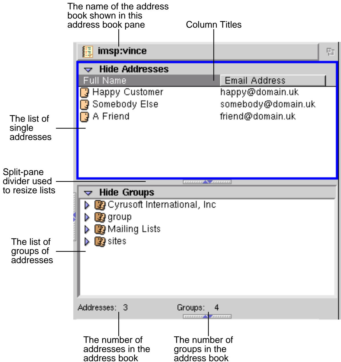
Figure 10 The Address Book pane
