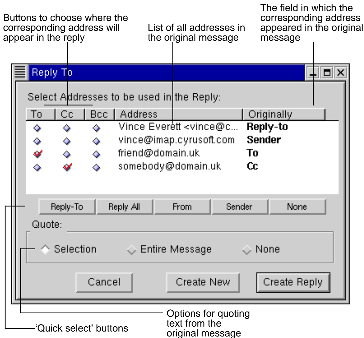
Figure 7 The 'Reply To' dialog
