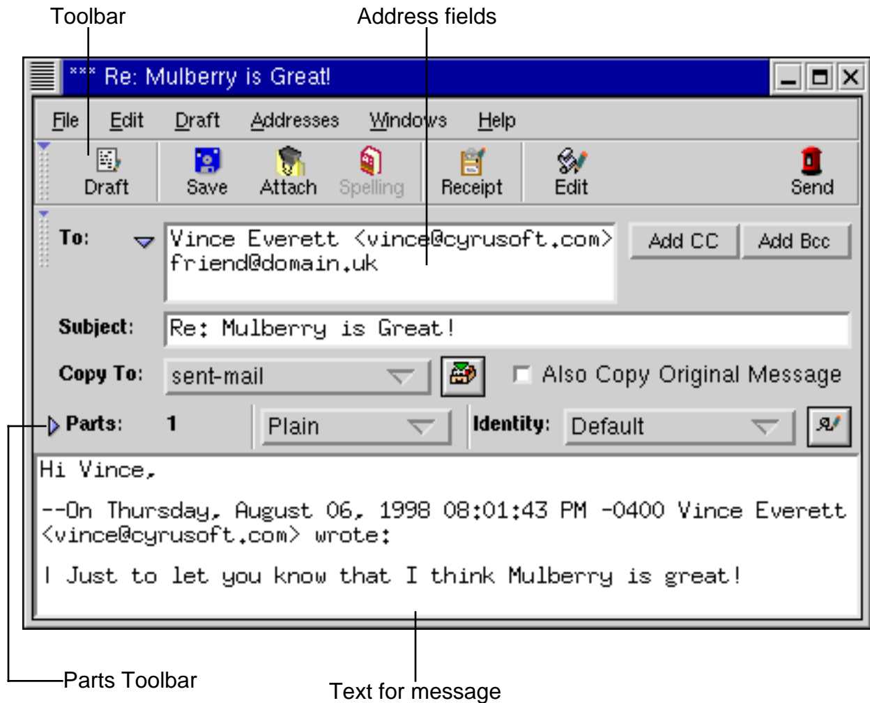
Figure 8 The Draft window
