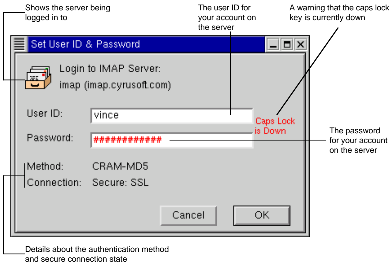
Figure 2 The login dialog
